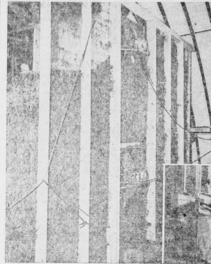
Air can be blown upward easily from the duct of a barn hay drier through only 5 or 6 feet of damp hay. Floating ducts installed during hay storage at the Pennsylvania State University Agricultural Experiment Station allowed air to reach all parts of the mow except the corners. Escaping air was measured as shown in the insert.
