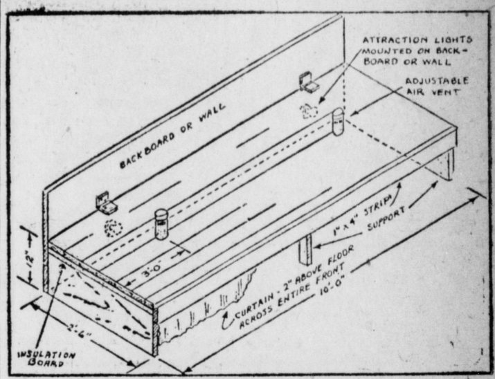
Shown above are specifications for a heating cable type of chick brooder.
