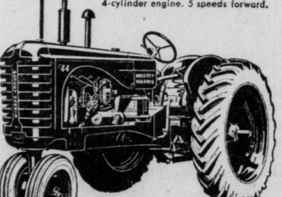
3-4-Plow "44"—260-cubic-inch, 4-cylinder engine, 5 speeds forward
