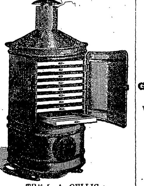
THE L. A. OELLIG DRY HOUSE, PATENTED JANUARY 21ST, 1869.
