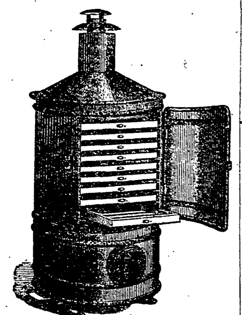
THE L. A. OELLIG DRY HOUSE, PATENTED JANUARY 13 th , 1863.
