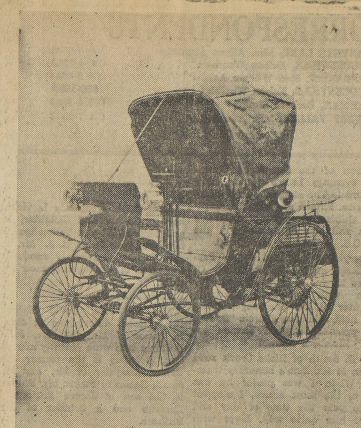
OLDEST CAR LURAY, VA.— One-cylinder, 5 horse power, hand starter, belt transmission, chain drive and solid tires are some of the specifications of this 1892 BENZ, the oldest car in America still in use.
