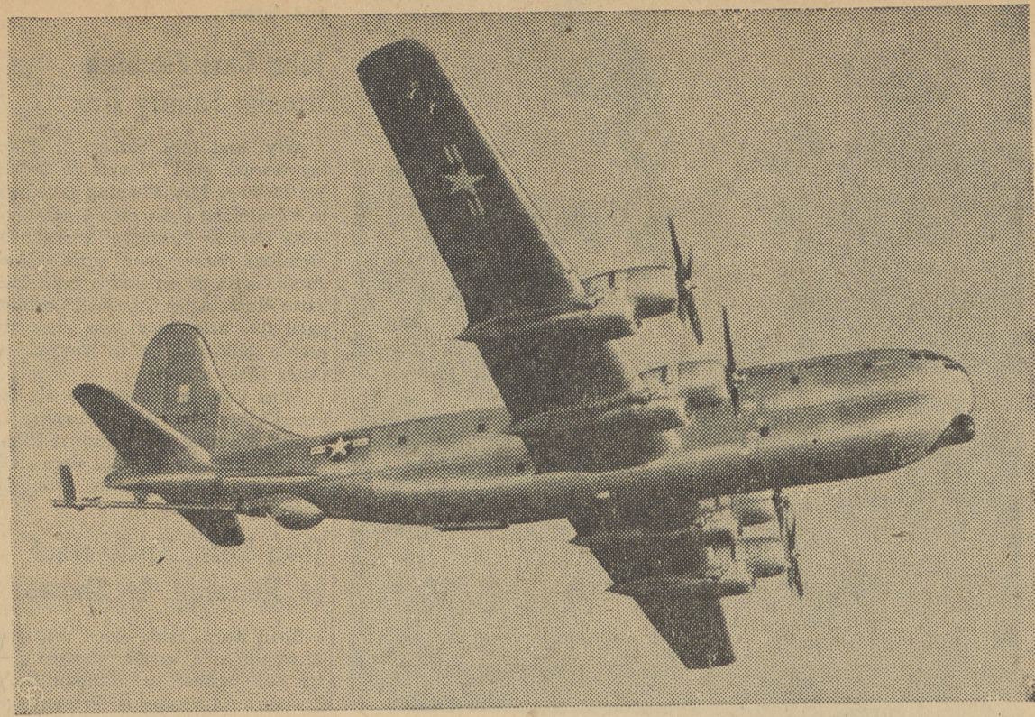
SHOWN DURING A TEST FLIGHT near Renton, Wash., is the new KC-97F Stratofreighter, big double-deck, multi-purpose plane which boasts a Flying Boom aerial refueling "pod." The Boom, used in various types of jet and piston-engine bombers, is a long, telescoping device controlled by "ruddervators" and operated from a control position in the under-belly pod. Now in large scale production, the Stratofreighters can be quickly converted from tanker to personnel, cargo, hospital or air re-supply purposes. (International)
