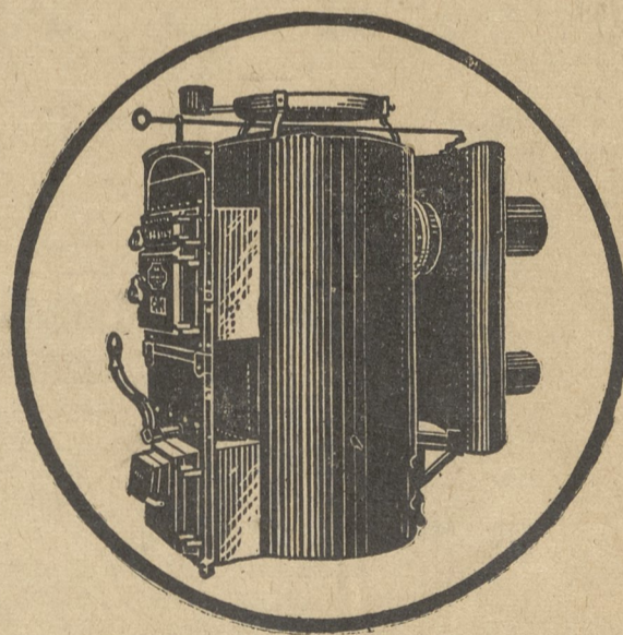
This shows the seamless steel furnace body with outer casing removed.
