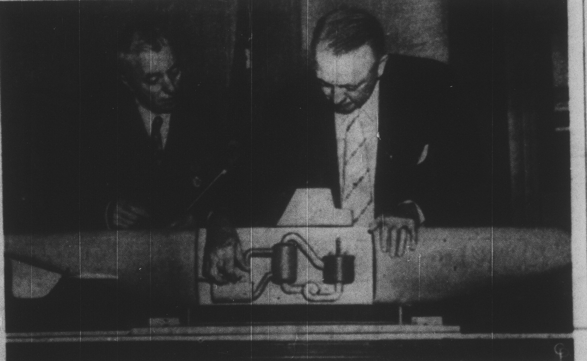
SECRETARY OF THE NAVY Dan Kimball (right) inspects in Washington a model of the first atomic-powered submarine. At left is its designer, Capt. Hyman George Rickover, who is explaining the arrangement of the atomic power plant in the craft. It was revealed that one pound of the submarine's nuclear fuel will generate as much power as 2,600,000 pounds of coal or 350,000 gallons of gasoline. Captain Rickover was given a second Legion of Merit award. (U. S. Navy—Defense Department Photo from International)
