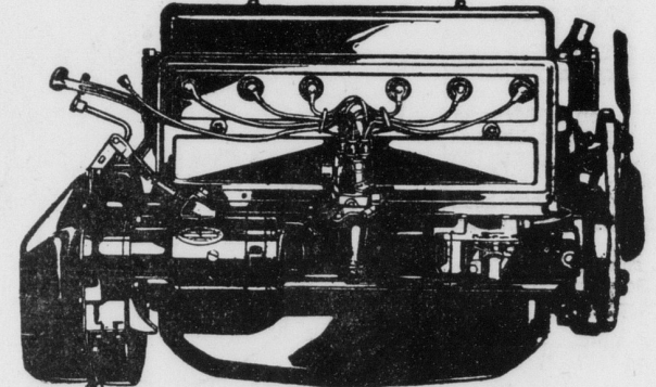
Chevrolet's new six-cylinder, fully enclosed valve-in-head engine has a high compression non-detonating head. Its piston displacement is 194 cu. in. and it develops 40 H. P. at low engine speed.
