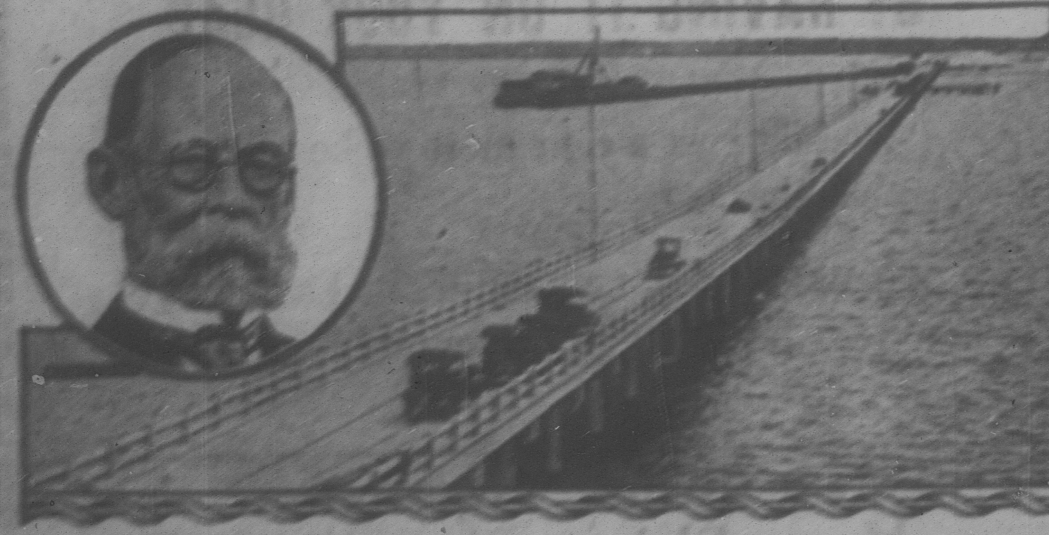
This is the longest toll bridge in the world, between St. Petersburg and Tampa, Fla., a distance of 24 miles. It is the longest toll bridge ever built in the world. The job in the beginning was to get it started. After 20 years ago, George & Gustav (brothers), after whom the bridge is named, saw the possibilities in such a project and obtained the right of way, but the work was begun in 1912 and the bridge is now completed.
