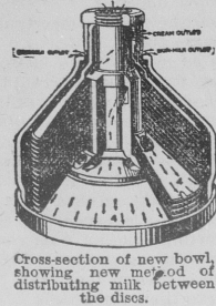
Cross-section of new bowl, showing new method of distributing milk between the discs.
