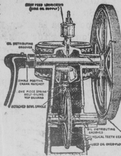
Showing automatic oiling of NEW De Laval.
