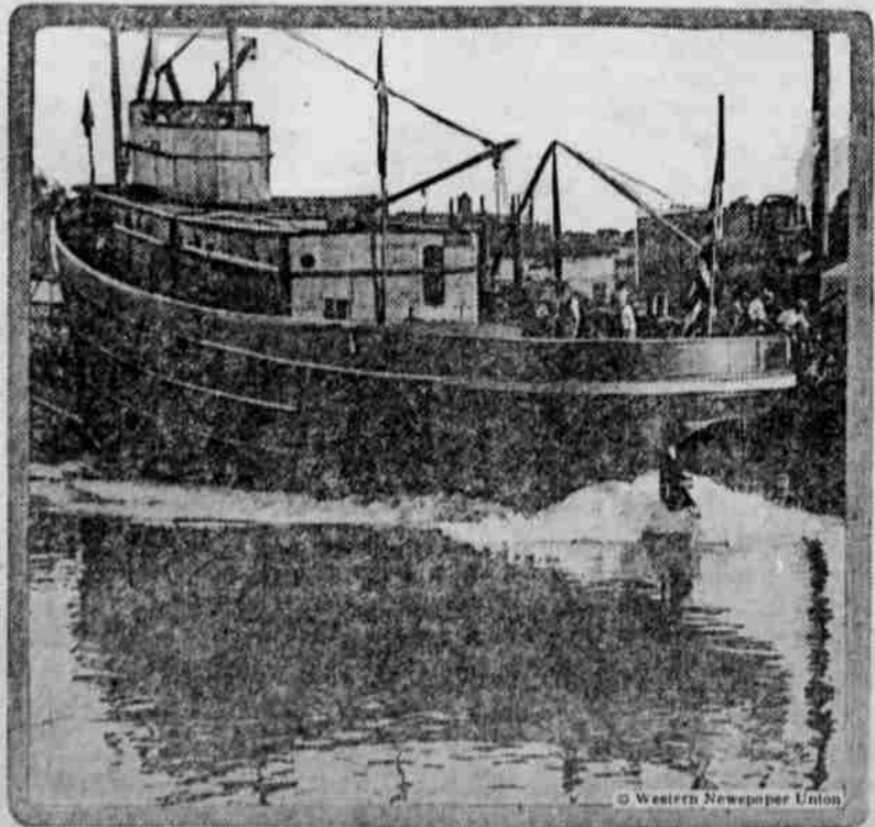
The Sanderling, fifth of a series of ten mine sweepers and layers contracted for by the Todd Shipbuilding company, taking to the waters at Brooklyn. The ship is 128 feet long, has 1,400 horse power and can make a speed of 14 to 15 knots an hour.
