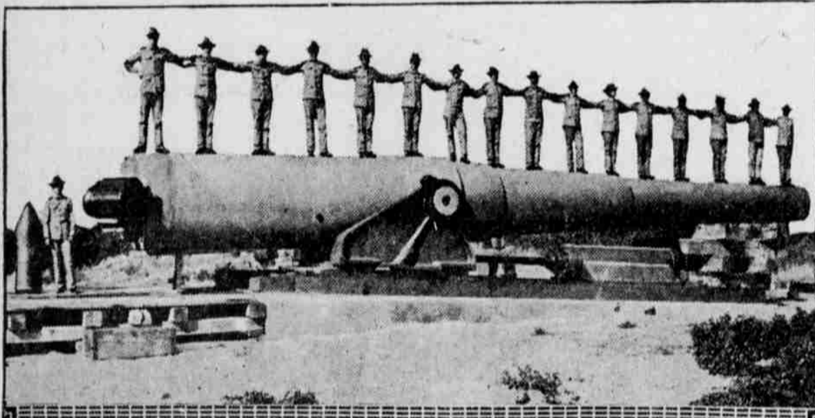
This, the largest gun in the world, has been made to defend the Pacific entrance to the Panama canal. It has a 16-inch bore, weighs 130 tons and throws a projectile weighing 2,400 pounds. The weapon will be mounted on a disappearing carriage on one of the small islands off the mouth of the canal.
