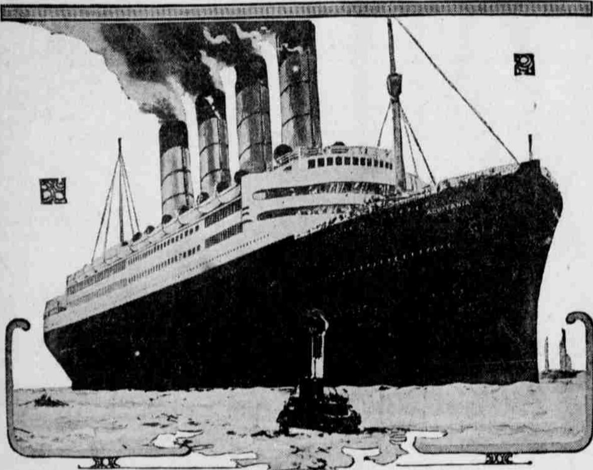
At Clydebank, Scotland, the steamship Aquetania, largest of the Cunarders, is being prepared for sea, having been launched last April. She is a ship within a ship, having absolutely water-tight inner and outer shells. Her dimensions show that she will be one of the largest ships afloat. She is 901 feet long, 97 feet wide, 92 1/2 feet deep to the boat deck. Her gross tonnage is 47,000 tons. She will have a speed of 23 knots an hour, and accommodations for 3,520 passengers and a crew of almost 1,000.
