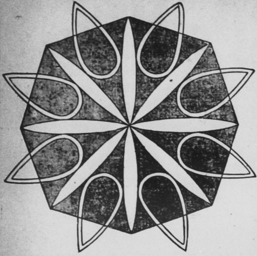
Without removing your pencil from the paper, trace every line without retracting or crossing any intersection.—N. Y. Herald.
