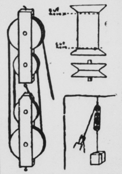
THE PARTS AND COMPLETED PULLEY.
