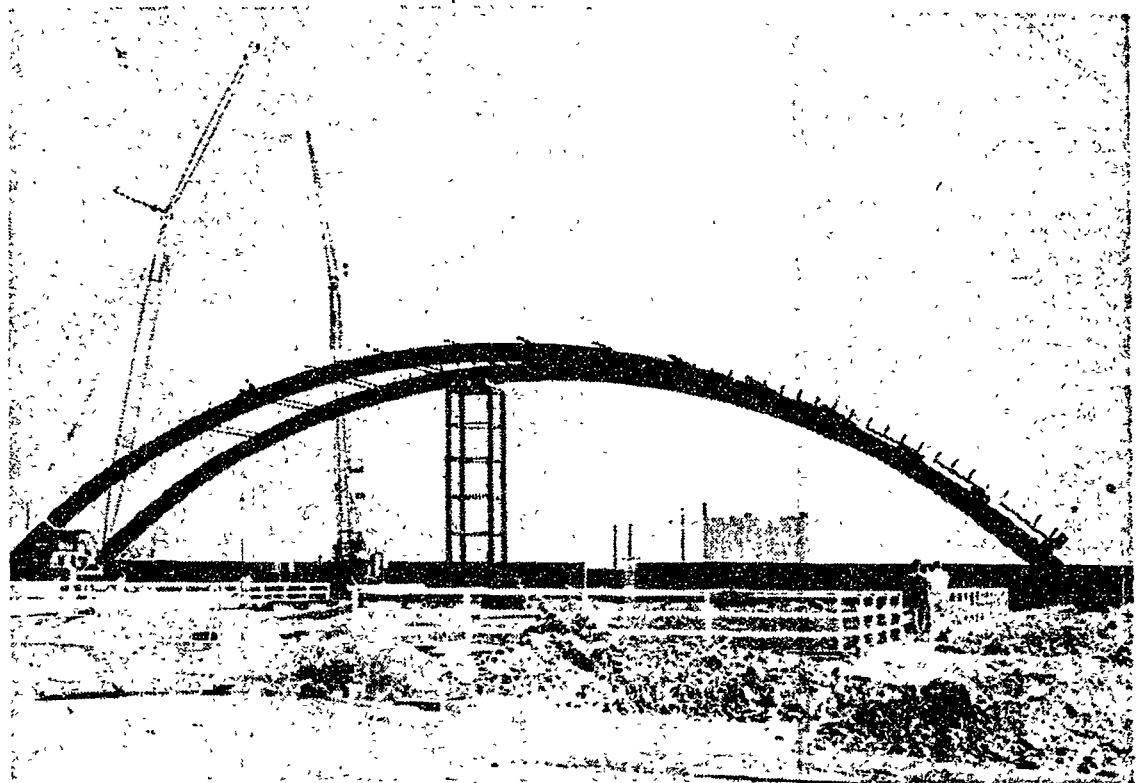
THE FIRST FEW ARCHES of a 9-arch span to cover the skating rink are now in place. The rink is 260 feet long and the spans are 198 feet from side to side. Each one weighs 30 tons and is shipped in four sections. Both ends will be open as well as the sides. The cover is to protect the rink from weather changes and is expected to add over 2 months to the skating season.
