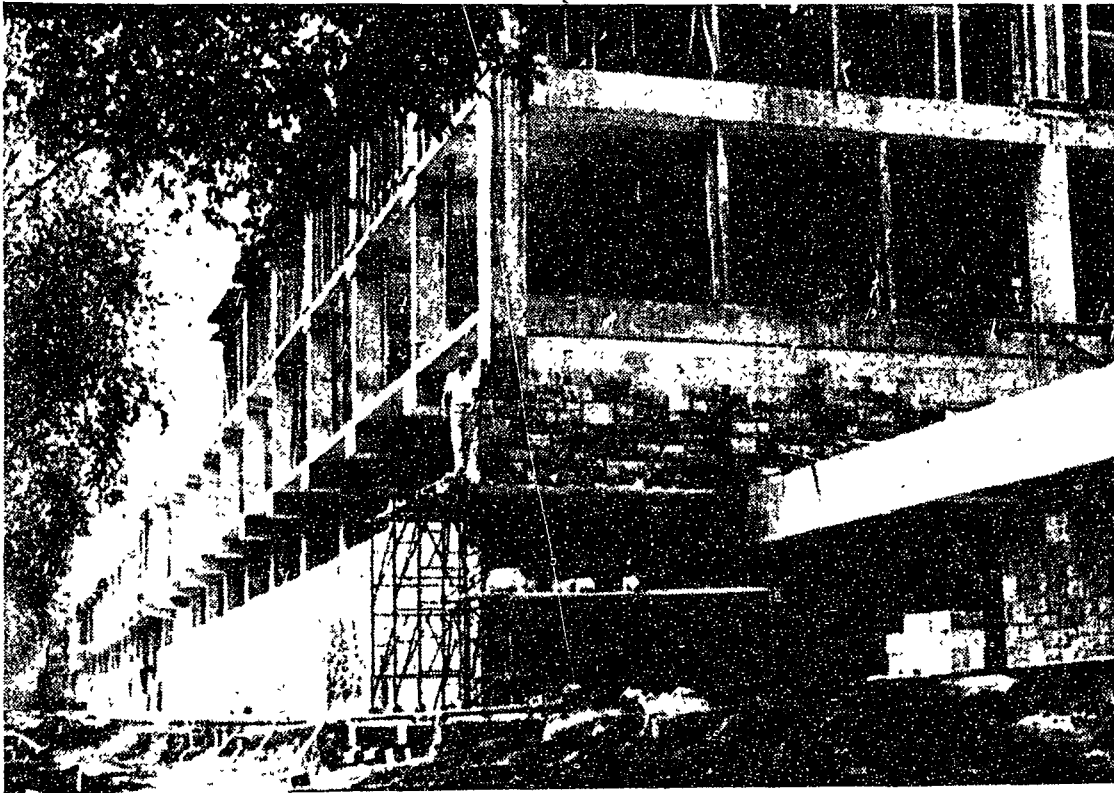
THE 690 FOOT LONG ENGINEERING BUILDING is about at the half-way point in completion. Builders are pouring concrete and placing the front of stone. Hammond Building is located between the Mall and Burrowes Road along College Ave.
