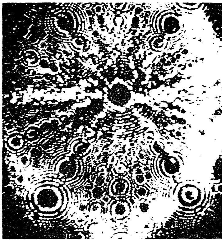
NAME THE SHAPE —It's a camera-shy scientific marvel snapped for the first time by Dr. Erwin W. Mueller, research professor of physics—the atom.
