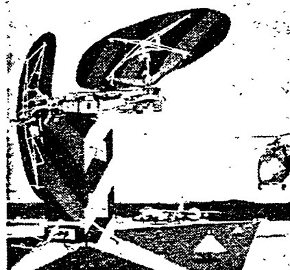
GILFILLAN GCA QUADRARADAR provides Search, Precision Final Approach, Height Finding and Airport Taxi Control in a single, air-transportable equipment. Designed for and highly efficient in handling military and civil jet aircraft, Quadraradar has received immediate and universal acceptance.
