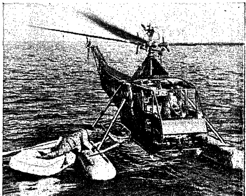
The helicopter, widely plugged as the post-war family air jalopy, has already been tested and found practicable by the Coast Guard as a means of rescue. Shown in demonstration by the Third Naval District's USCG Air Arm, "water-bug-like" copter settles near "wounded" man on life raft. Breezy-but-safe basket attached to fuselage is for the extra passenger.
