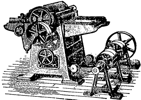
No. 2 Planer and Matcher.
