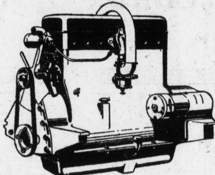
6 cylinders, 3 3/8 in. bore x 5 1/2 in. stroke
