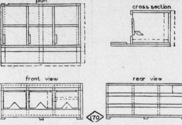
HOW TO MAKE A THREE SECTION TRAPNEST COPYRIGHT, 1915.
