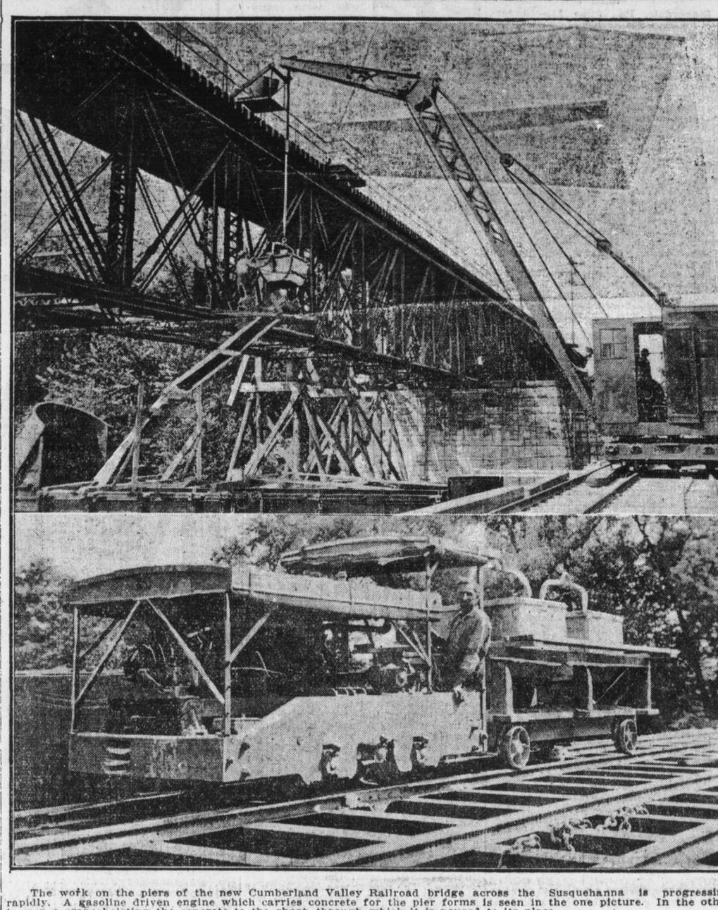
The work on the piers of the new Cumberland Valley Railroad bridge across the Susquehanna is progressing rapidly. A gasoline driven engine which carries concrete for the pier forms is seen in the one picture. In the other is seen a crane hoisting the concrete to the shoot, through which it is poured to its place.
