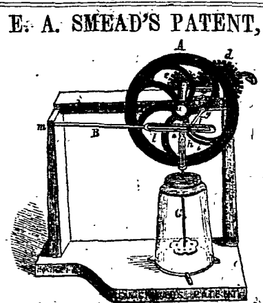
For Converting Rotary into Reciprocating Motion, and Vice Versa.
