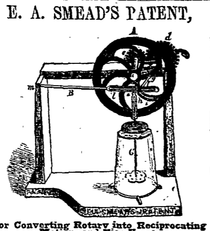
E. A. SMEAD'S PATENT, For Converting Rotary into Reciprocating Motion, and Vice Versa.
