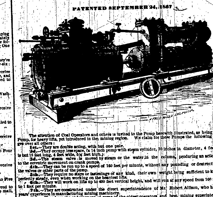
ALLISON CATARACT STEAM PUMP, FOR MINES, ROLLING MILLS, WATER WORKS, &c.
