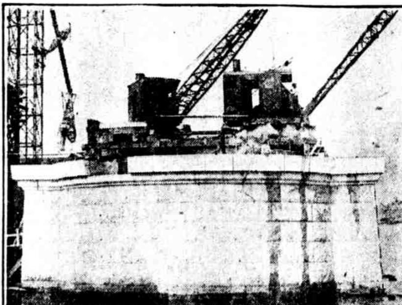
THE START OF THE PHILADELPHIA PIER for the Delaware River Bridge at the foot of Vine street. Two derricks handle the huge blocks that make up the new construction
