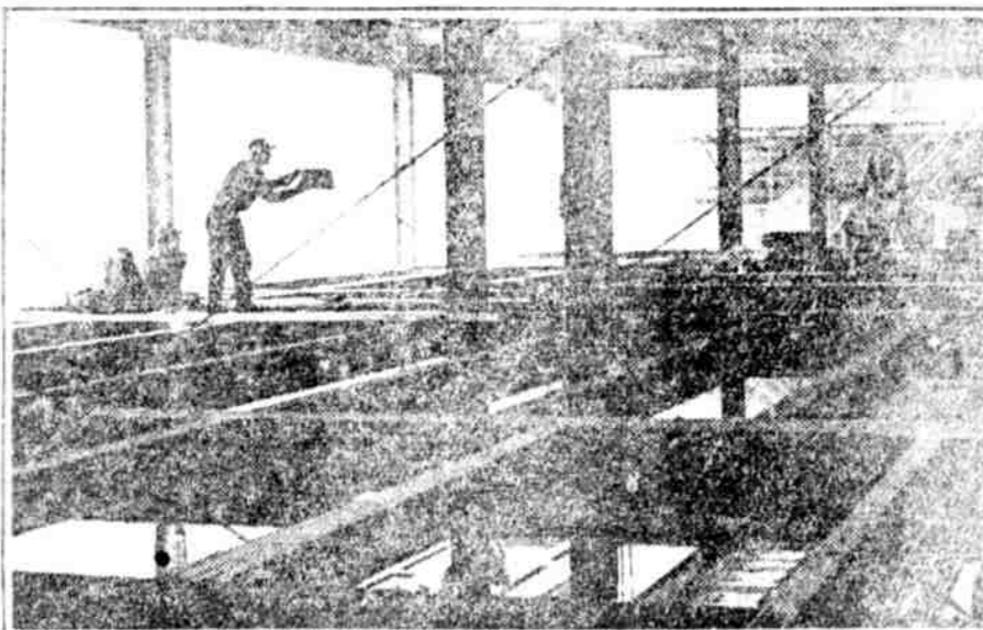
"SHOOTING" THE RIVETS. On the third floor of the new office building at Seventh and Chestnut streets. The workman at the right is operating the furnace and "shoots" the hot rivets to the "catcher."
