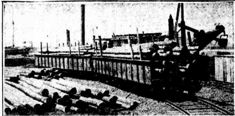
TIMBER FOR PILING IS ARRIVING BY RAIL AND WATER AT KAIGHN'S POINT, CAMDEN. Soon work will be started on the building of the mammoth Philadelphia and Reading Terminal. Steam shovel in the background is clearing the way. The man in the boat is getting the piling together.
