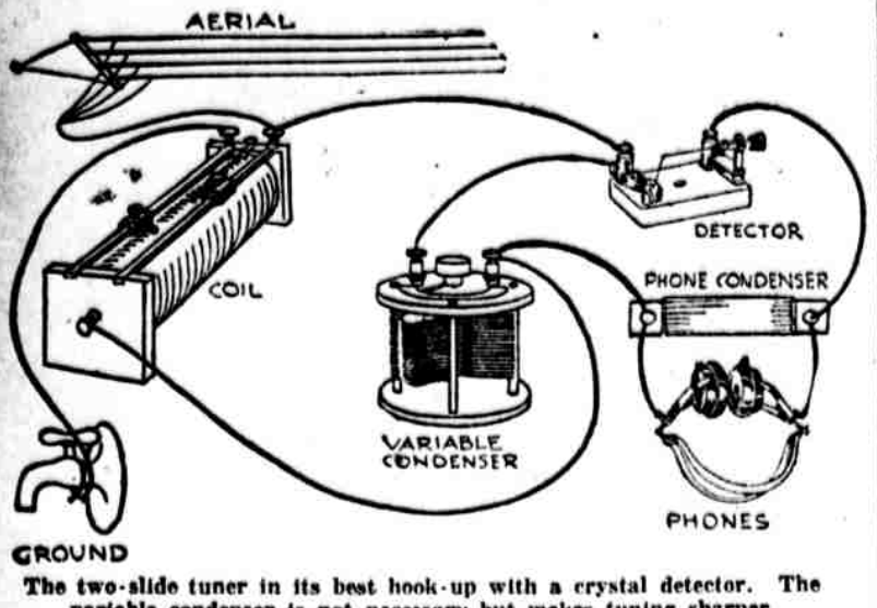
The two-slide tuner in its best hook-up with a crystal detector. The variable condenser is not necessary but makes tuning sharper.
