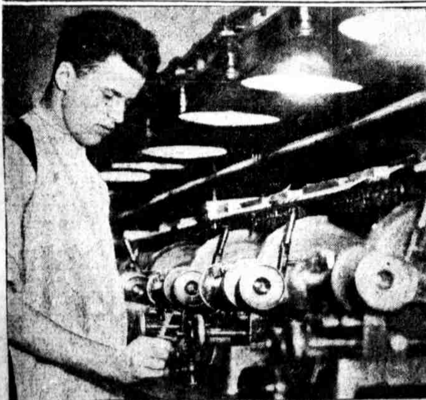
WILLARD RICHTER, Yeaton, Pa., operating spectacle and eyeglass lens-grinding machine at the workrooms of Wall & Ochs, opticians, 1716 Chestnut street.
