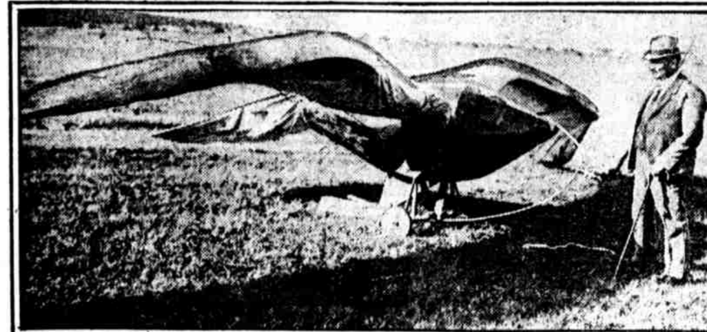
AN ENGINELESS AIRPLANE or "glider," such as recently exhibited in Germany. The plane, invented by Karl Rath, is built on the lines of a hawk, the large bent wings being filled with compressed air to hold them rigid. Wide World
