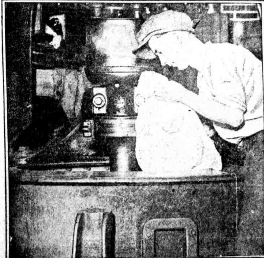
HIZZING OUT THE MOISTURE at the Oxford Dye Works, 1410 East Ford street. Oliver Kerr, of 1357 East Palmer street, handles 6000 pounds of dye a day in this machine, which operates by centrifugal force. L. P. S.
