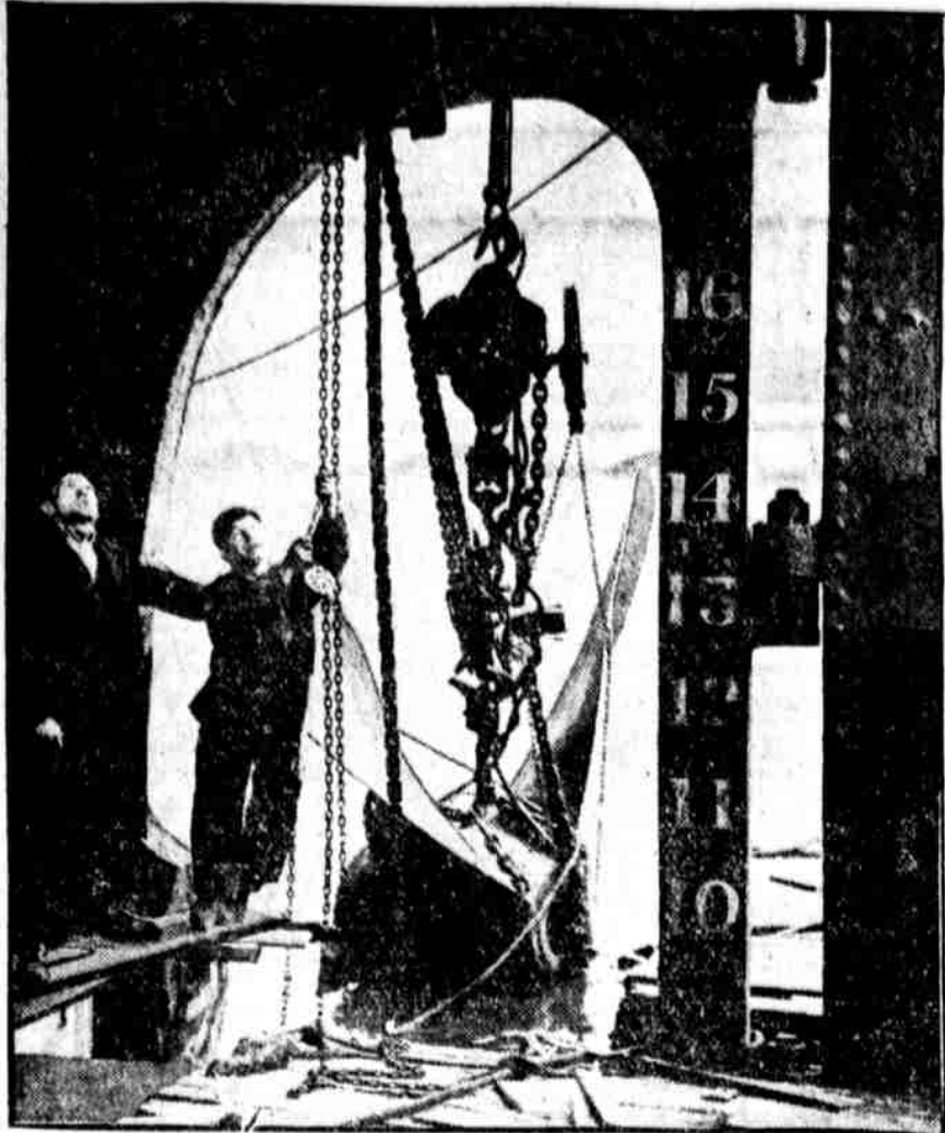
PLACING NEW PROPELLER. The steamship Baylula, at Pier 38, South Wharves, was towed in from sea with a broken propeller. Drydocks are few, so the repair work goes on, as the stern of the ship is lifted out of the water by heavy loading of the front part.
