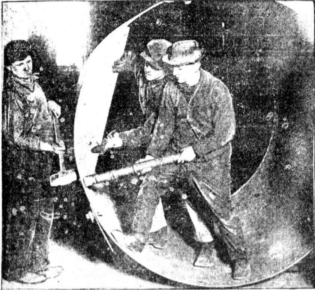
ROUNDING BOILER PLATE INTO CIRCLE. William M. and William B. and Jim Wellington detaching the first rivets into the hole after cutting this section of boiler plate. They are workers in the Keystone Boiler Works, 6140 Columbia street.
