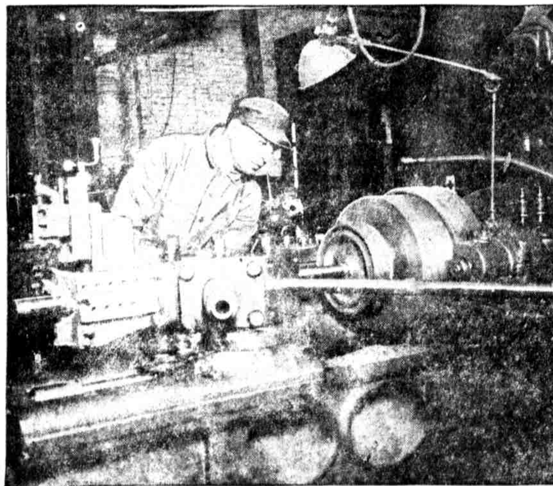
TURNING DRIVING PULLEYS FOR BOX-W ASHINES. Walter Wunderlich, 4346 North Third street, Philadelphia, guiding the boring bar on a lathe at the plant of the Stokes & Smith Manufacturing Co., Summerdale, Pa.
