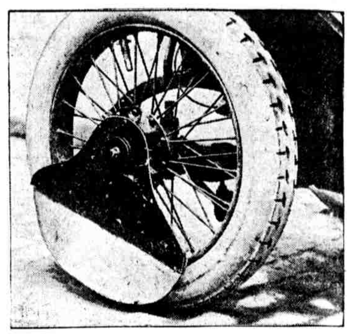
PREVENTS SPLASHING MUD ON YOUR NEW DRESS. A Paris wheel device designed to collect the mud and shoot it backward on a line with the car. Kadel & Herliet.
