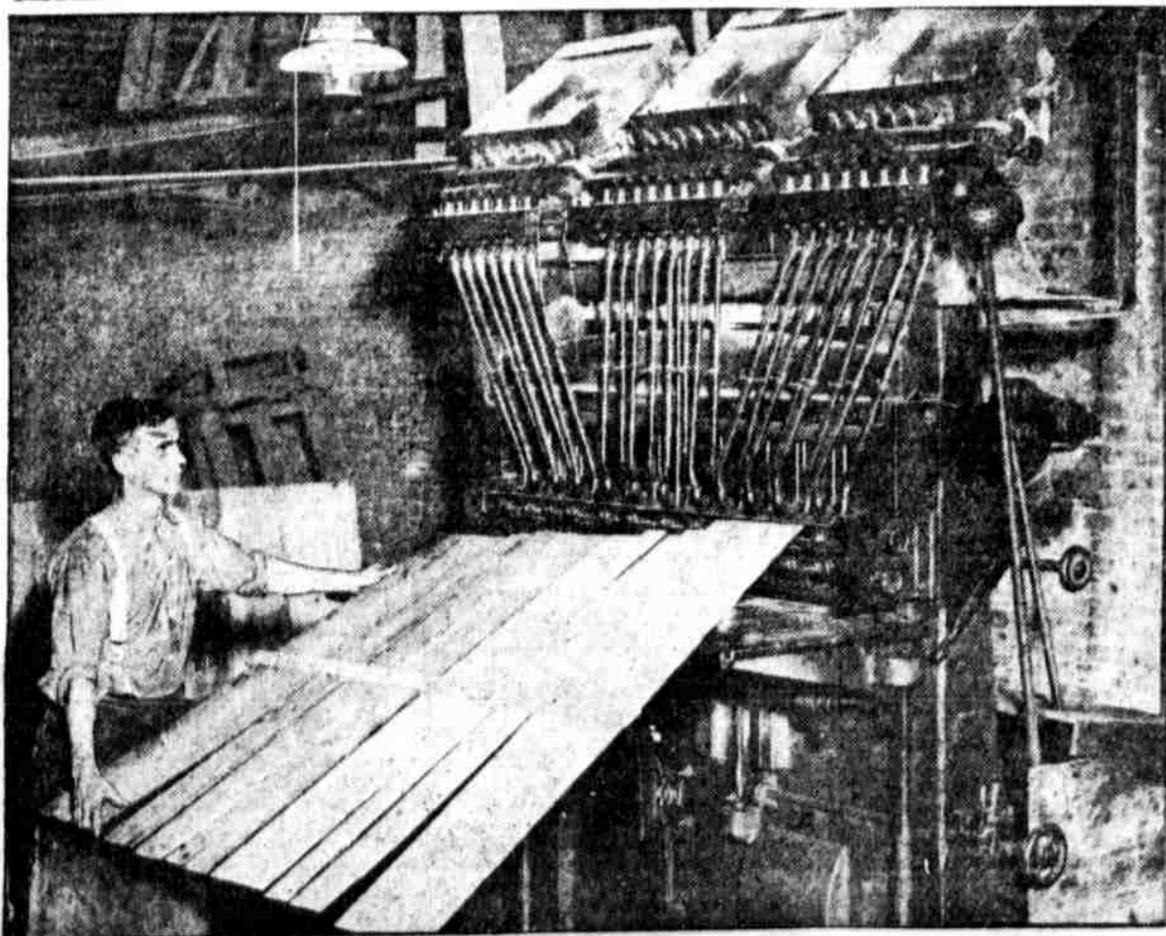
THOMAS GILMORE, 1263 South Bonsall street, is operating a nailing machine at the William J. Kee manufacturing plant, 111-117 North Orianna street. In putting the bands and battens on the large boxes, the machine drives twenty-four nails at a time.
