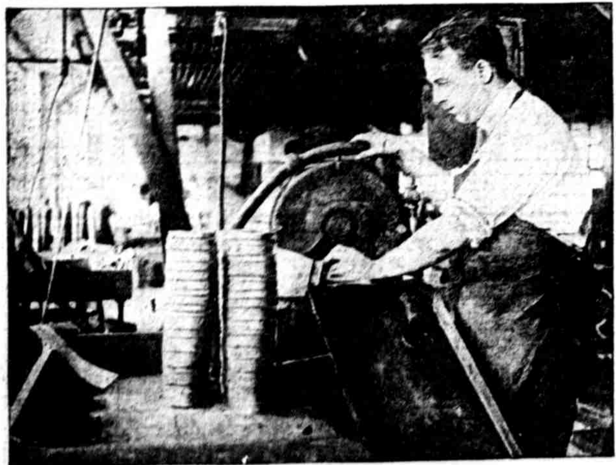
A. A. JOHNSON, 1822 ARCH STREET, operating a machine at the Wilkening Manufacturing Co., between and Mt. Vernon streets, that does side grinding of piston rings at the rate of 5000 a day.
