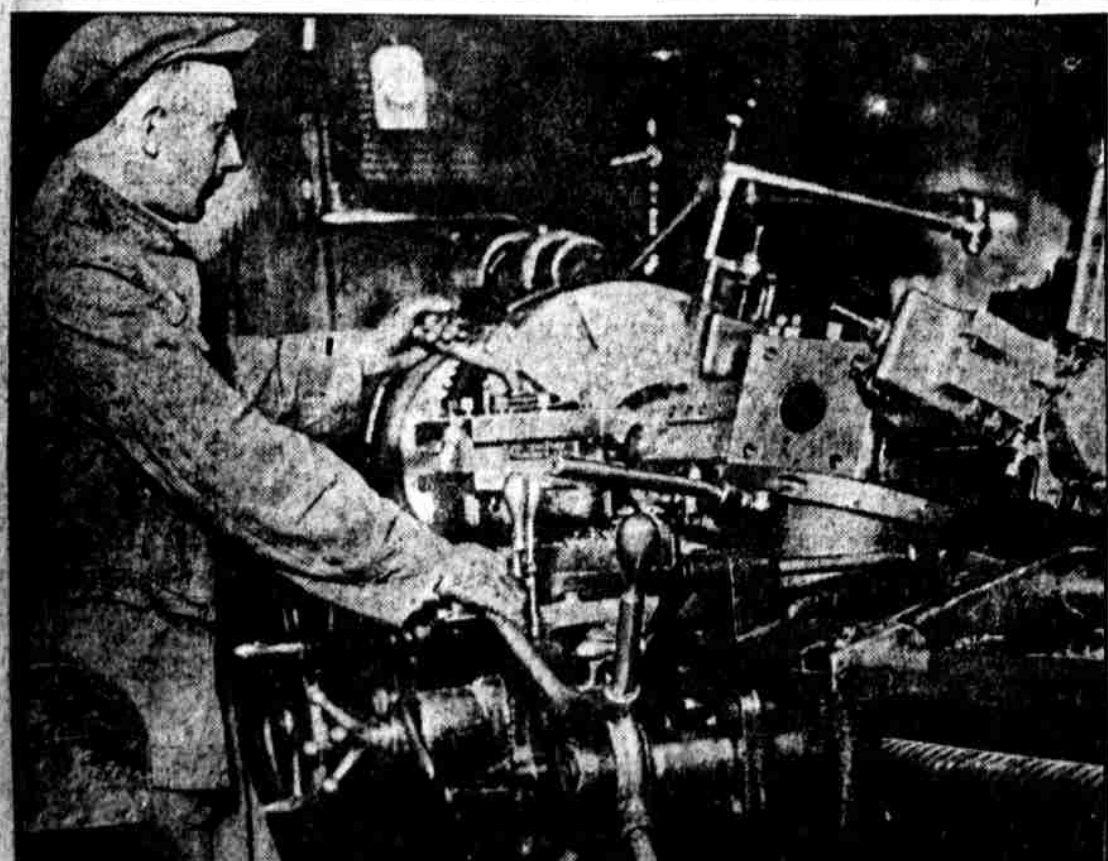
WILLIAM SCHMIDT, 1610 St. Luke's street, operating a turret lathe at the Hess-Bright Manufacturing Co., Front street and Erie avenue. He runs sixty-five rings, used for ball bearings, through the machine each day.
