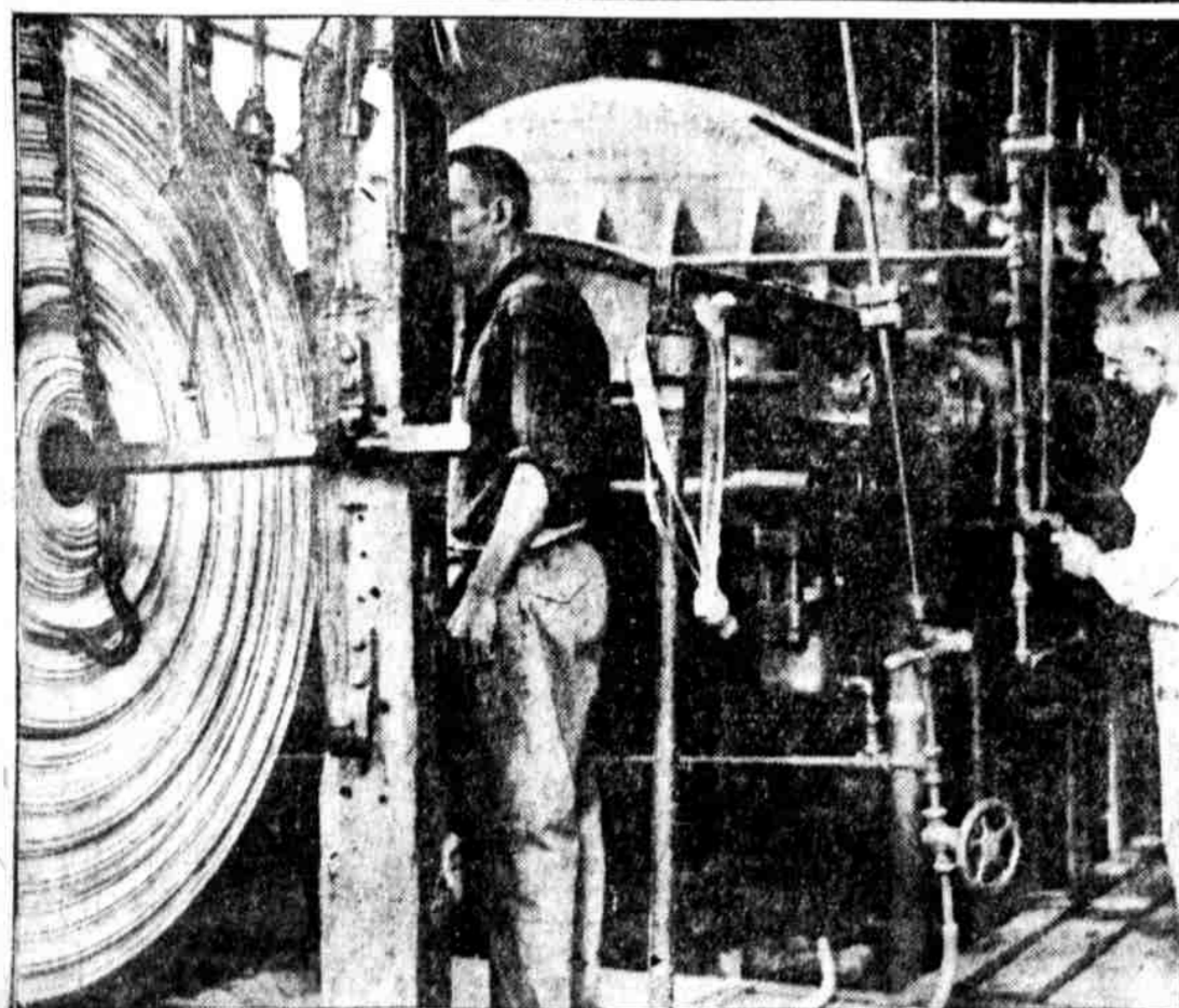
BELT PRESS. This machine vulcanizes the belt, which is the finishing touch in the manufacture of rubber belting, at the Quaker City Rubber Co., Wissinoming. Long rolls of cotton duck have previously been impregnated with rubber and built up of several thicknesses. Nicholas Canning, 2032 Bridge street, and Philip Gaul, 619 Tioga street, see that the proper temperature and pressure are maintained. Ledger Photo Service
