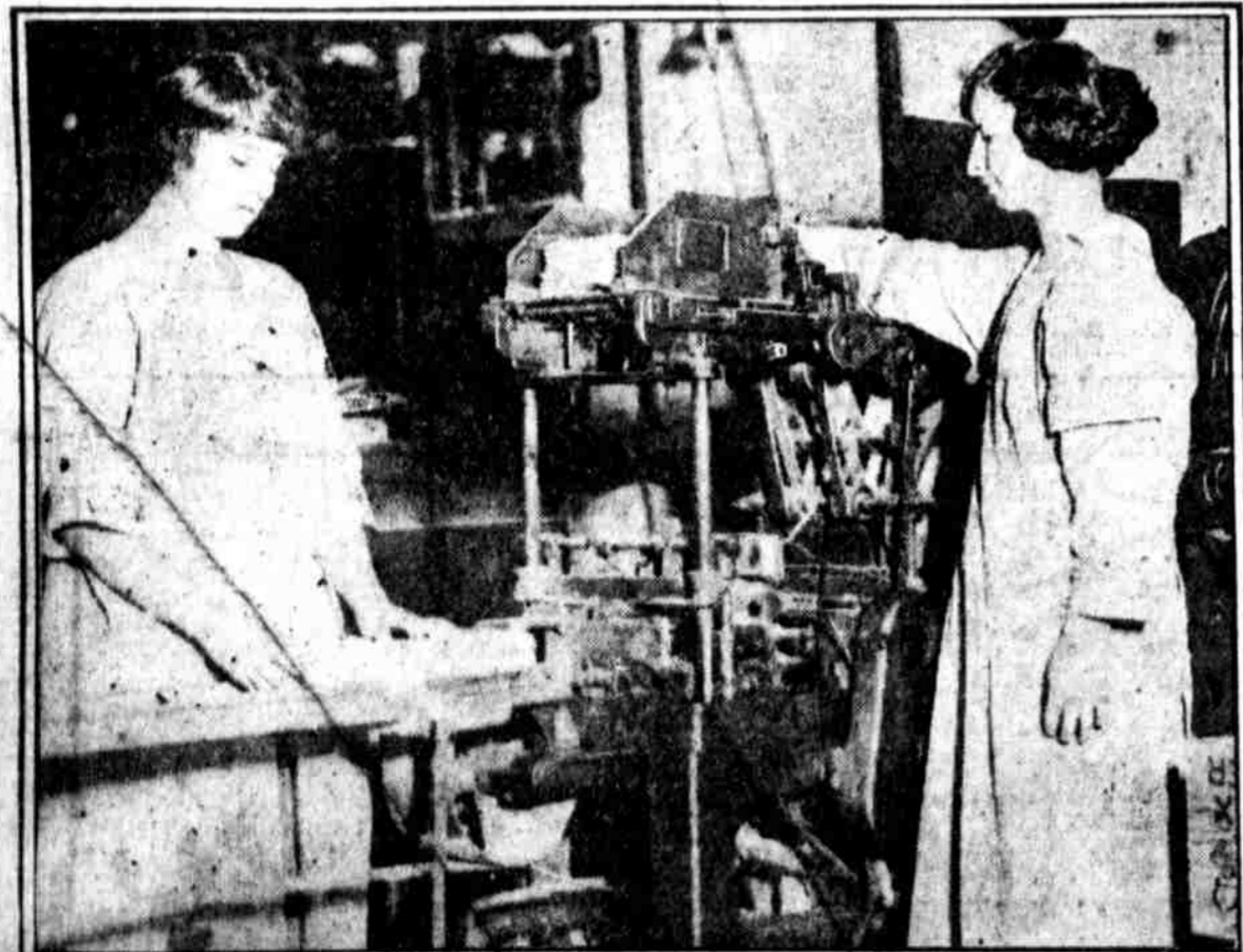
THIS MACHINE PLACES THE INNER AND OUTER WRAPPER ON CAKES OF SOAP at the Charles W. Young & Co., soap manufacturers, 1247 North Twenty-sixth street. It has a capacity of 64,000 cakes a day. The operators are Miss Emma Brenner, 2423 Seybert street (left), and Miss Elizabeth Hanley, 858 North Tansy street Ledger Photo Service
