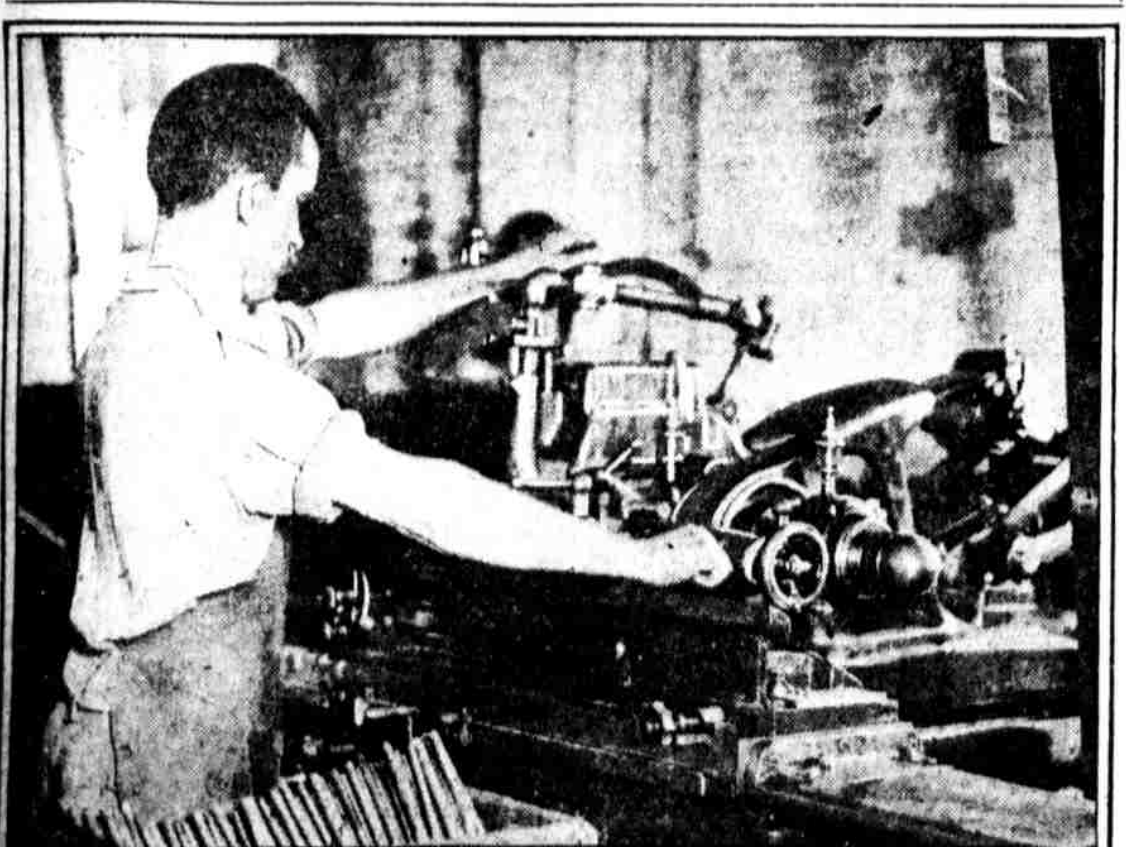
MAKING SPINDLES. George L. Bishop operating a machine at the Wicaco Screw and Machine Works, Seventh and Wood streets. Seventy-five of the 7-inch spindles are completed each day. Each one has four taperings, necessitating four different operations on this machine
