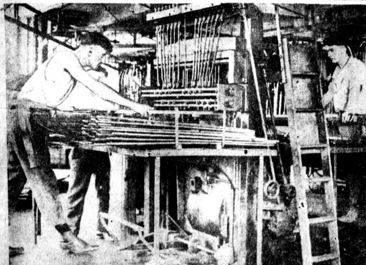
MAKING SLEDS. Joseph Wilson, 3732 North Marshal street (left), and Richard J. Partridge, 3939 North Franklin street, operating a nailing machine at the S. L. Allen & Co. plant, Fifth street and Greenwood avenue. In this operation the sled tops are being nailed to the sled frames at the rate of 2500 a day.
