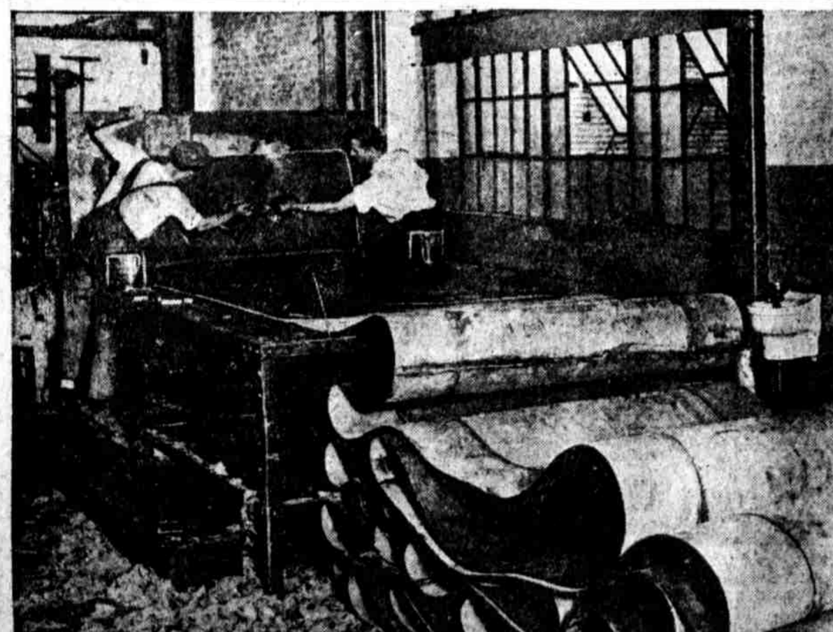
BUILDING A MACHINE BELT at Alexander Brothers, Third and Callowhill streets. This belt will weigh about 3000 pounds, necessitating the hides of 670 heavy steers. It will be tested to run a mile a minute, transmitting 1000 horsepower.
