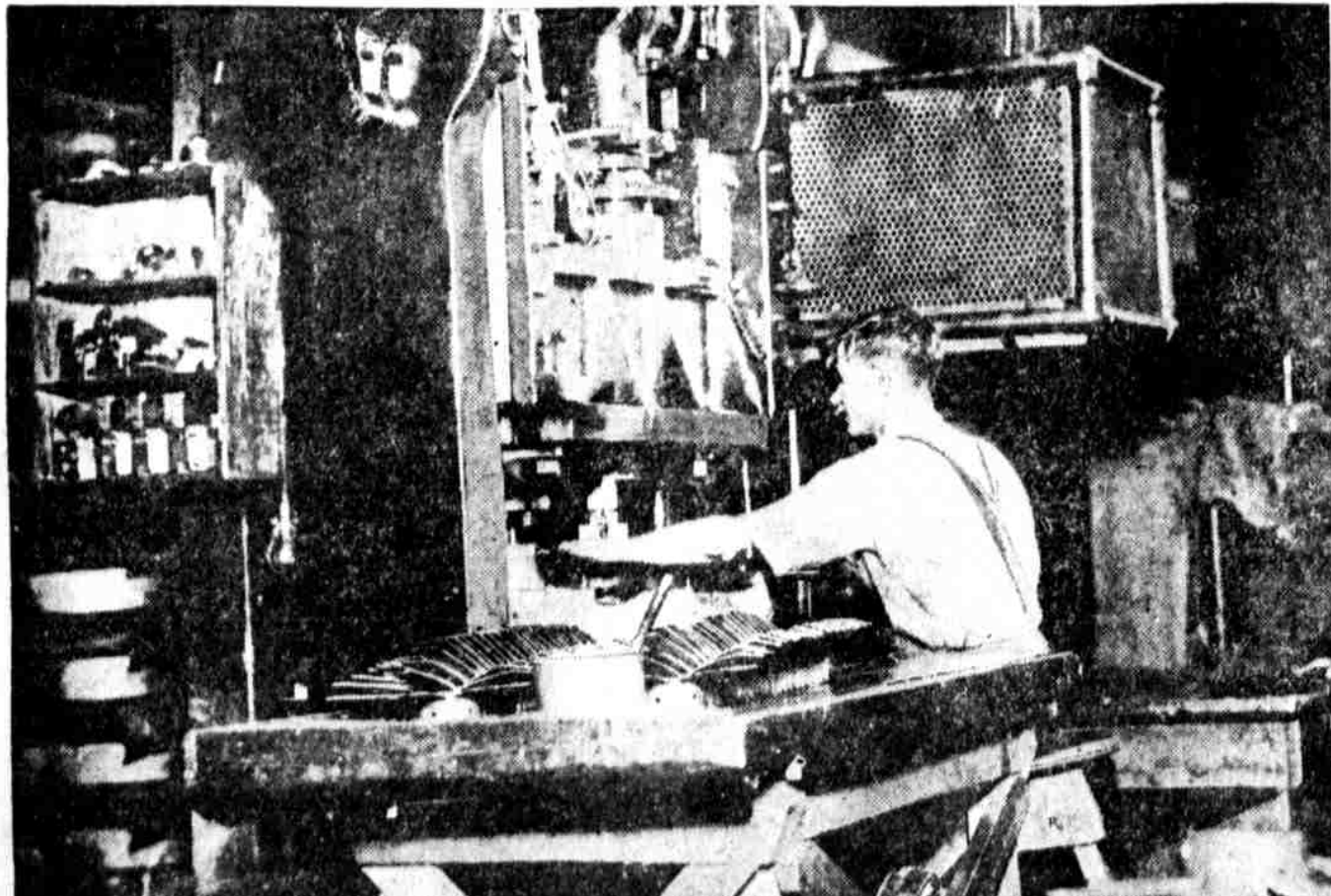
PIERCING SPIDER ARMS used on steel pulleys. A. Paslowki, 1926 East Dounton street, is operating the machine at the American Pulley Co., 4200 Wissahickon avenue.
