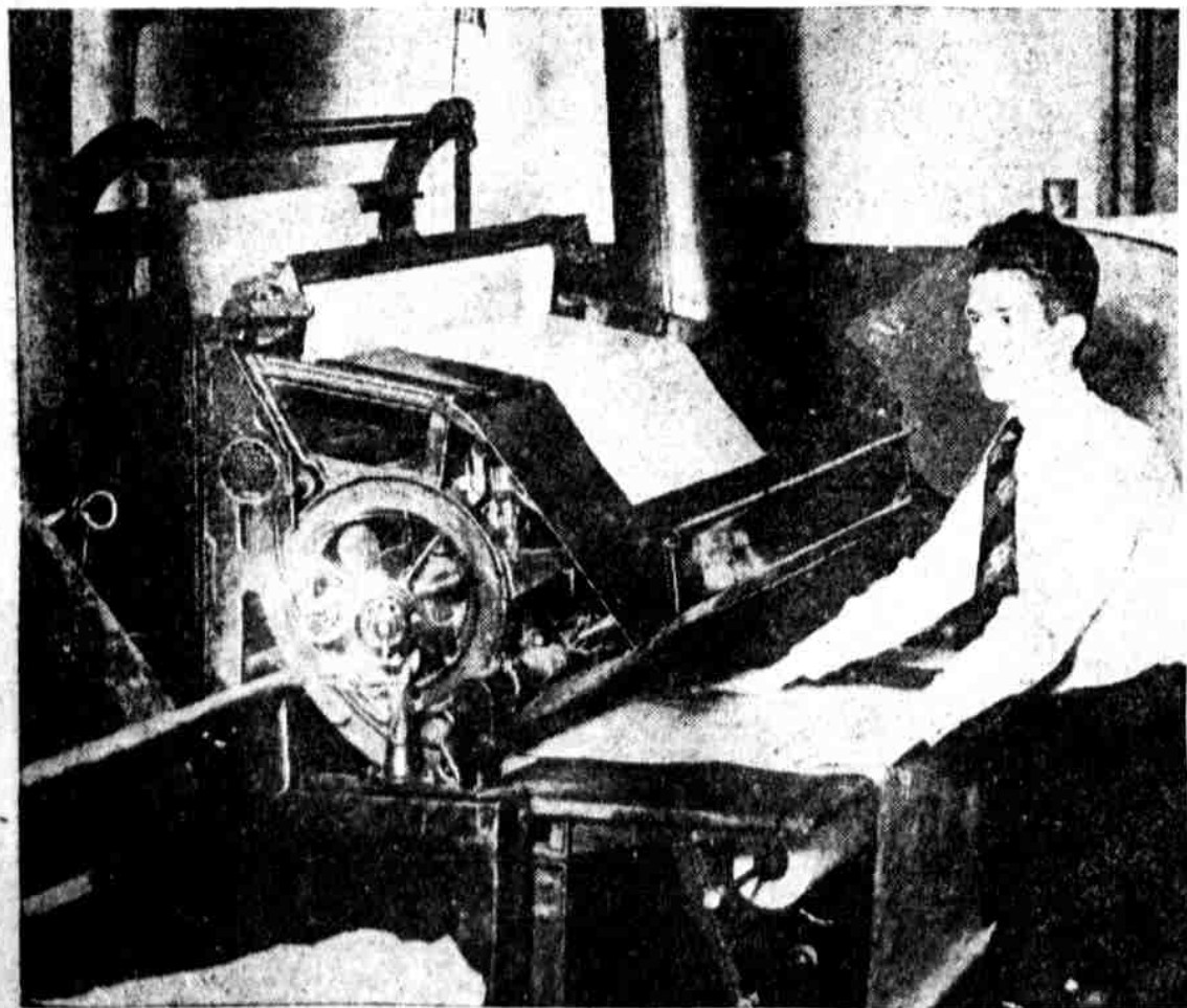
ELMER POLLOCK, 87 Sharpnack street, operating a blue-print machine at the General Reproduction Co.'s plant, 140 North Broad street. Thirty-six hundred feet of blue print are printed on this machine each day. Ledger Photo Service.
