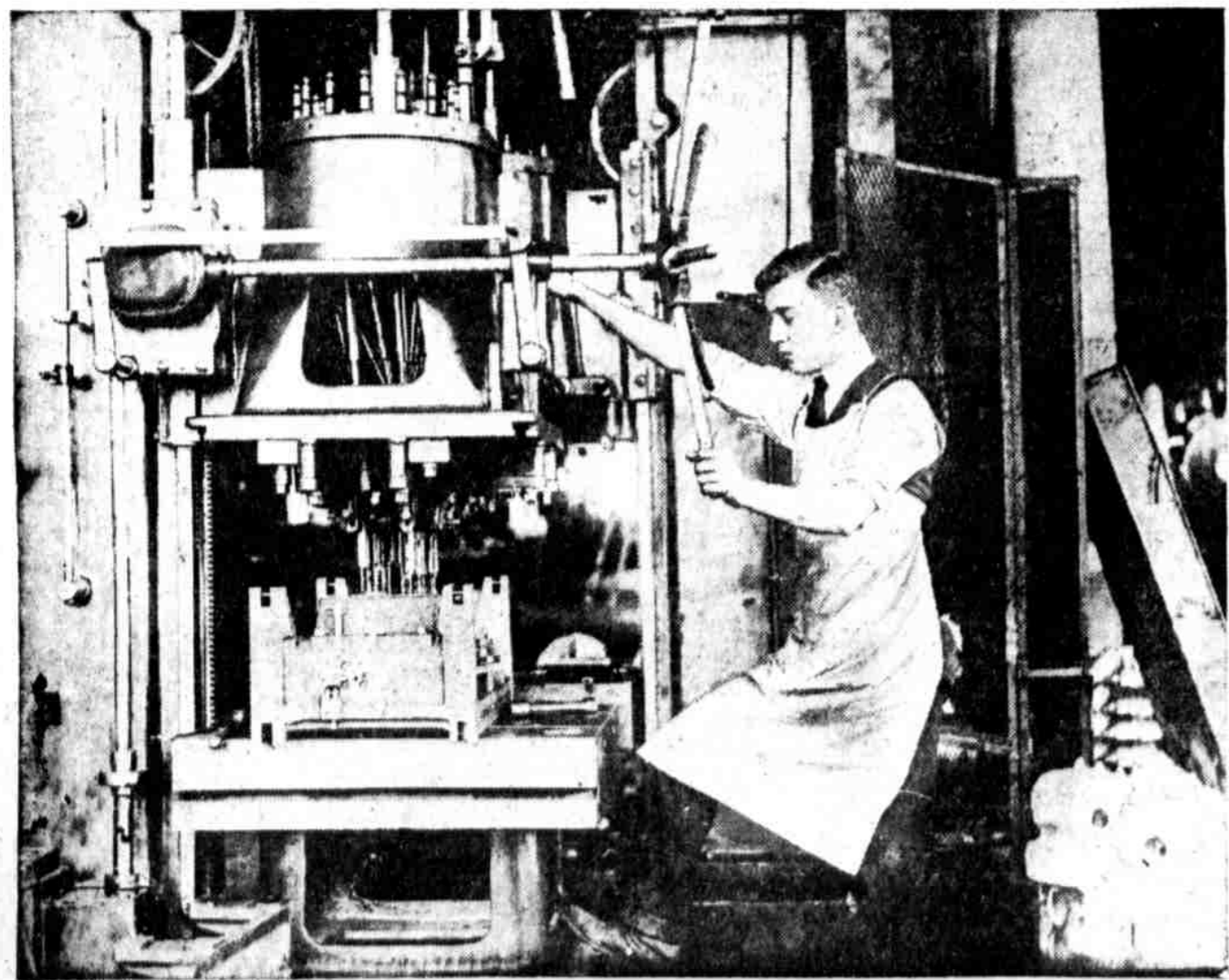
IRA WILLIAMS, 1626 South Yewdall street, operating a multiple drill at the Ace Motorcycle Corporation, Erie avenue and Sepviva street. Twenty-two holes are drilled in the same time in crank cases. Seventy-five of the crank cases are finished daily
