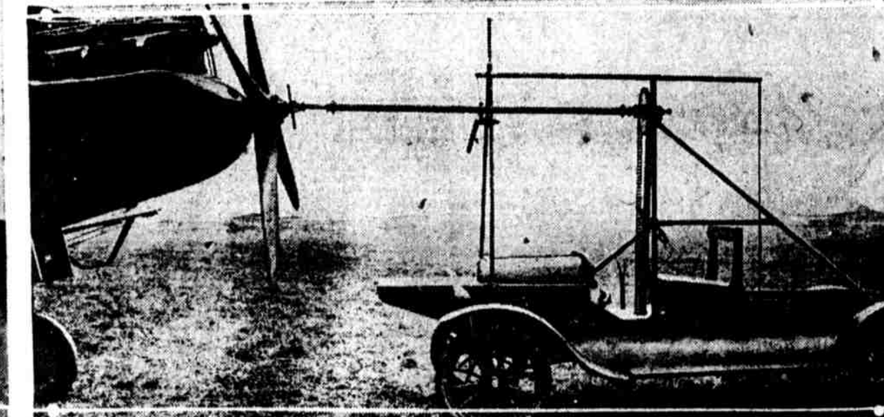
AN AIRPLANE ENGINE STARTER attached to engine of an automobile, originated by Captain B. C. Hucks, a British pre-war pilot.
